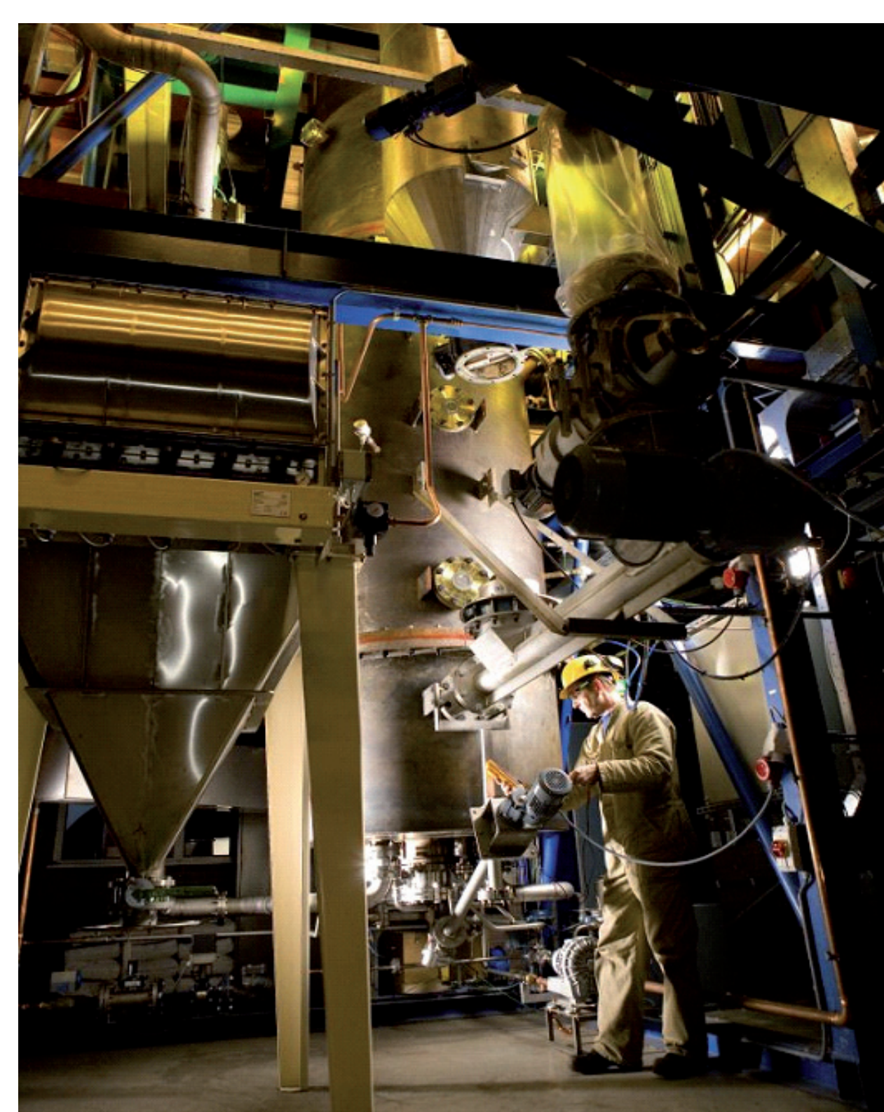
1 MW MILENA at ECN
