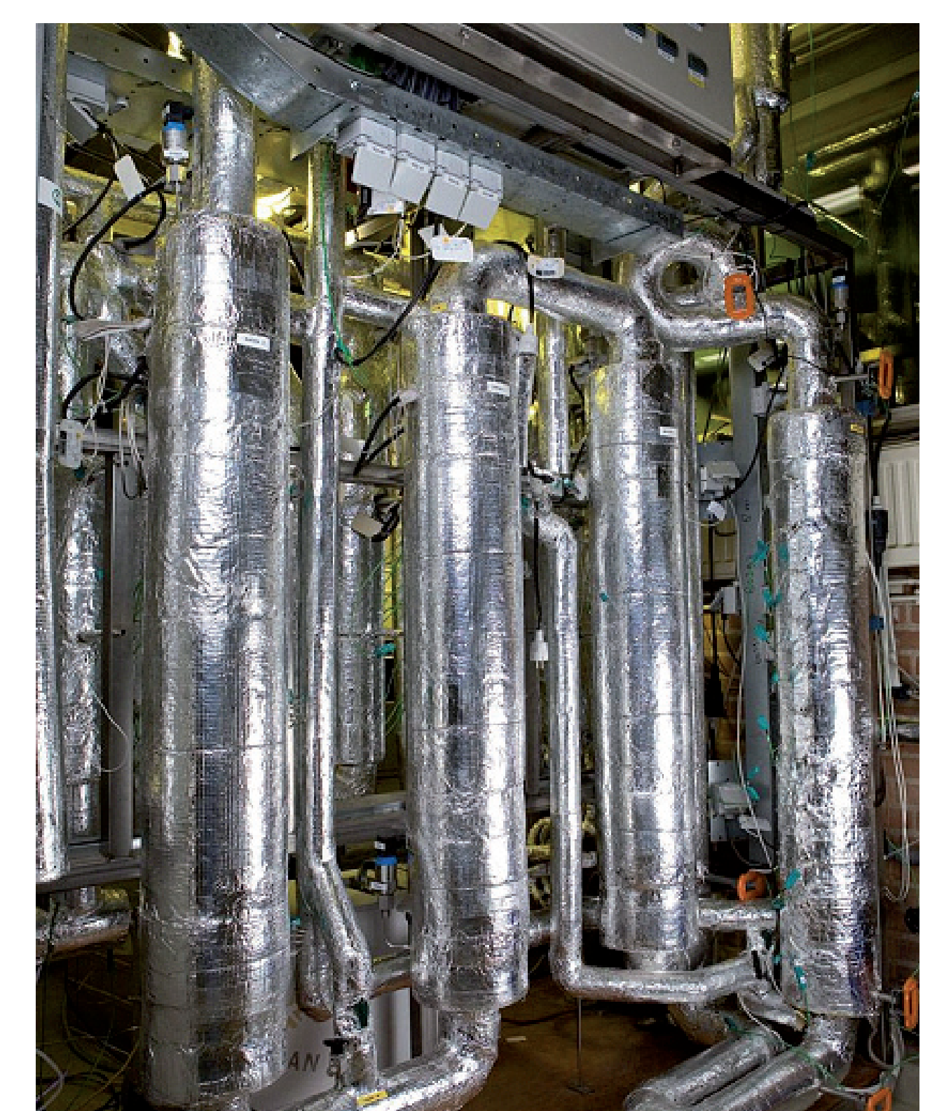
30 KW system for further gas cleaning and methanation at ECN
